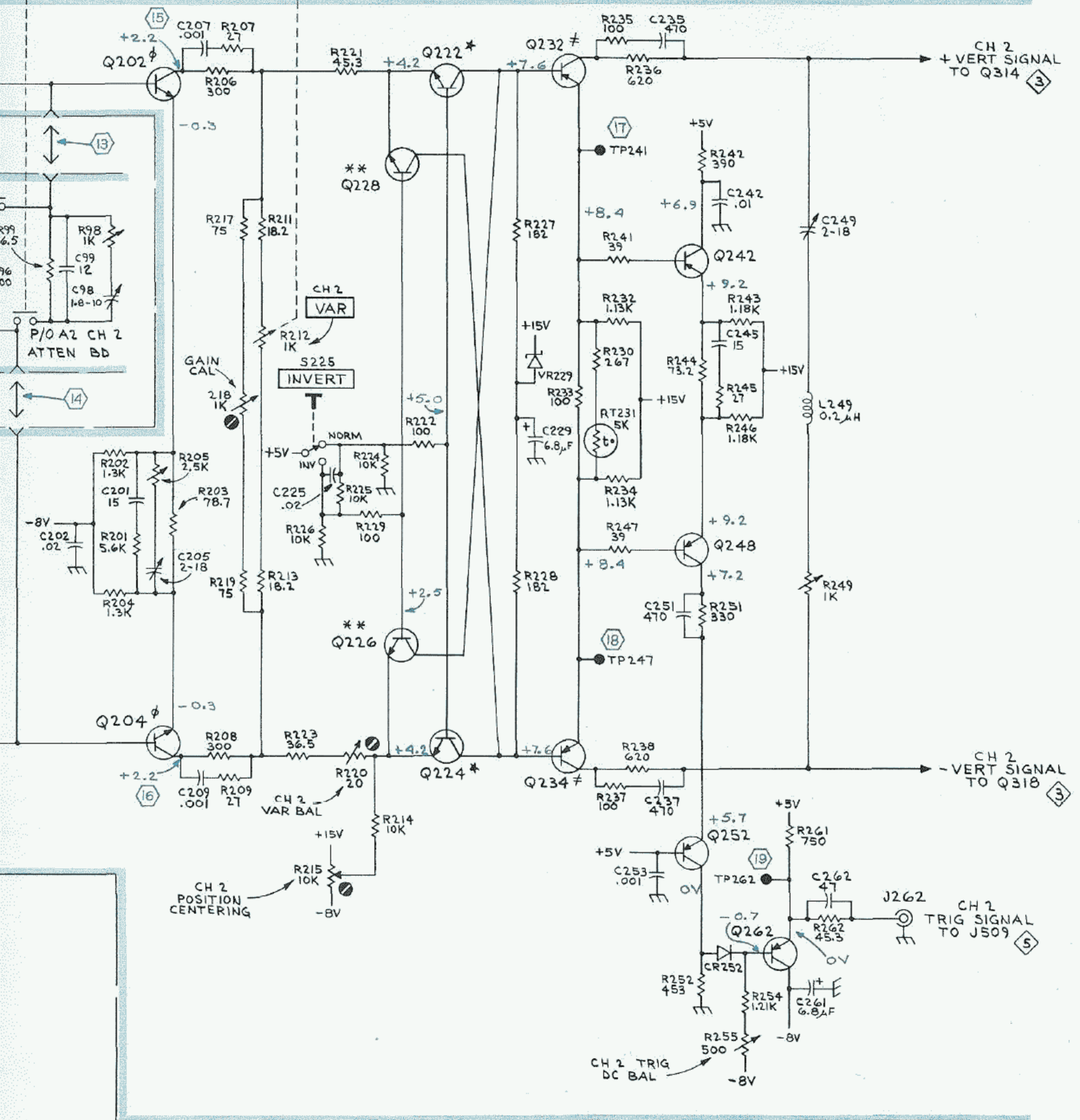
CH 2 VERTICAL PREAMP 2
