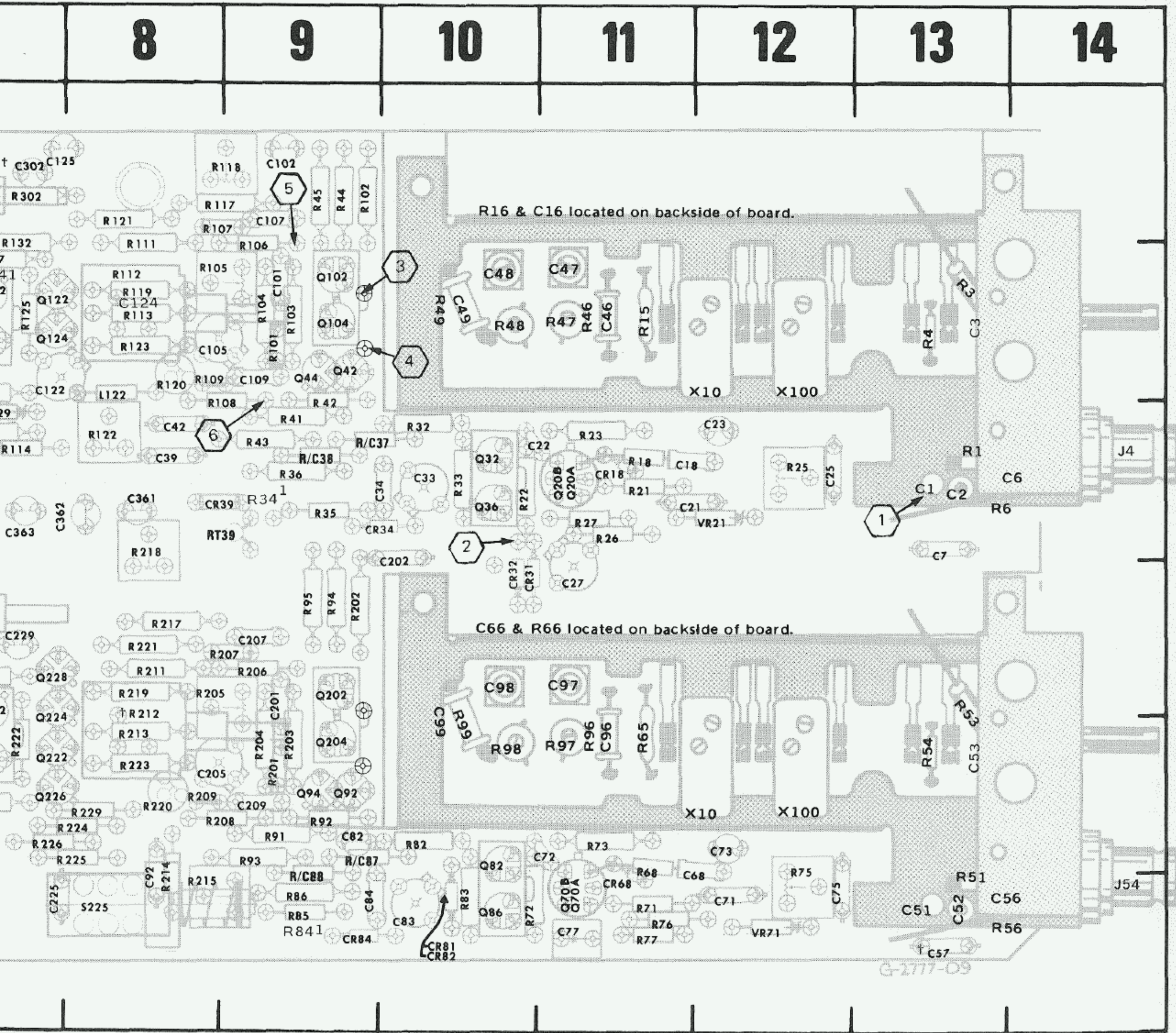
Resistors and A3—Vertical Preamp circuit boards.
